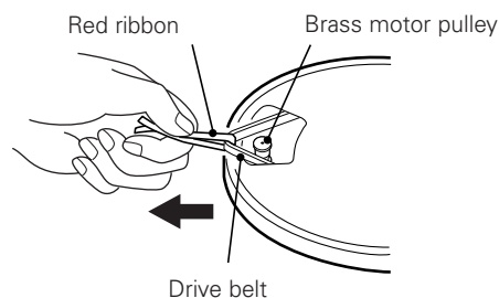
Figure 2 – Assembling the turntable
