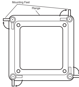
Diagram 6: Mounting Feet
